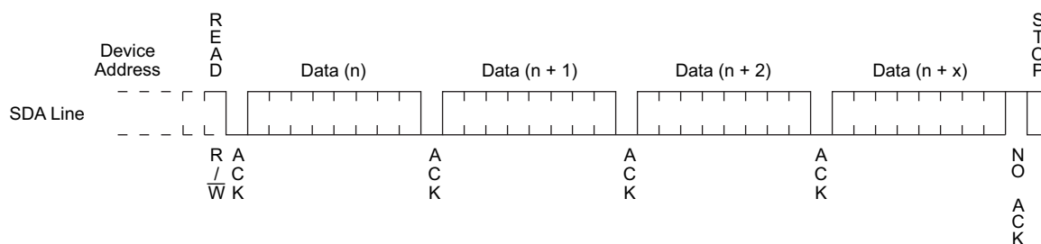
Figure 9-6. Sequential Read
