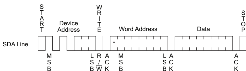
Figure 9-2. Byte Write
