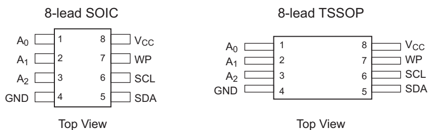
Figure 1-1. Pinouts
