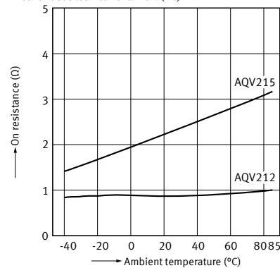
2-1. On resistance vs. ambient temperature characteristics
