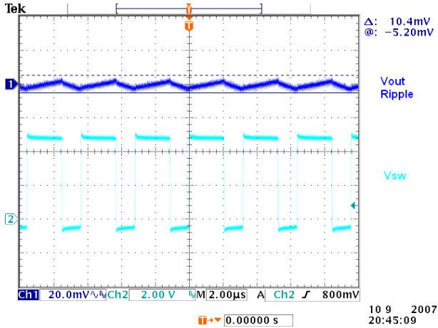
Vout Ripple (VIN = 5V, VOUT = 3.3V, IOUT = 0.1A)
