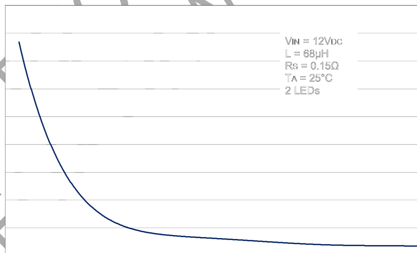
Figure 32 Low Duty Cycle PWM Dimming at 300Hz
