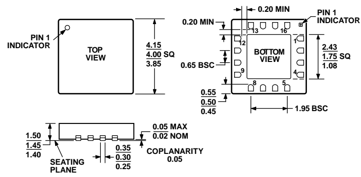
*STACKED DIE WITH GLASS SEAL. Figure 33. 16-Lead Lead Frame Chip Scale Package [LFCSP_LQ] 4 mm × 4 mm Body, Thick Quad (CP-16-5a*) Dimensions shown in millimeters
