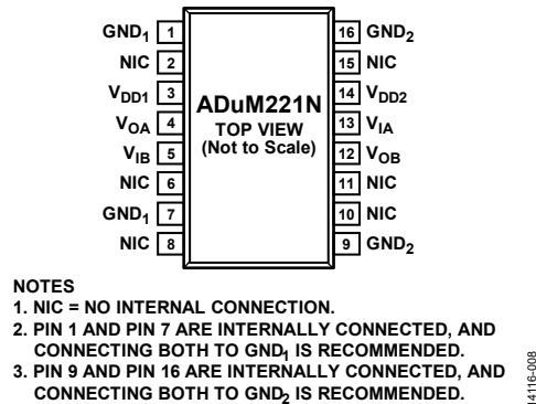
Figure 8. ADuM221N Pin Configuration
