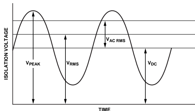
Figure 23. Critical Voltage Example
