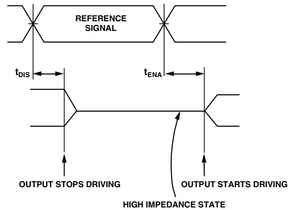
Figure 62. Output Enable/Disable
