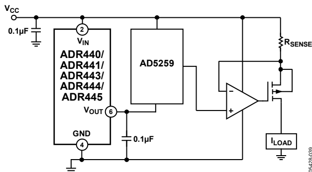
Figure 38. Programmable Current Source
