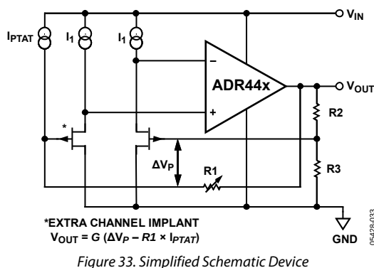
Figure 33. Simplified Schematic Device
