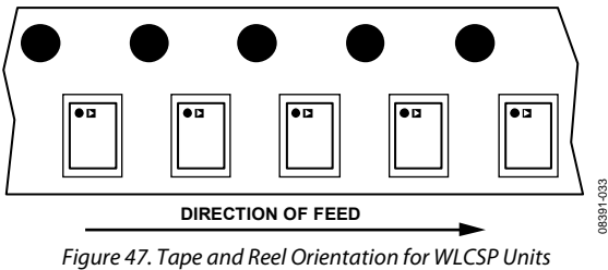
Figure 47. Tape and Reel Orientation for WLCSP Units
