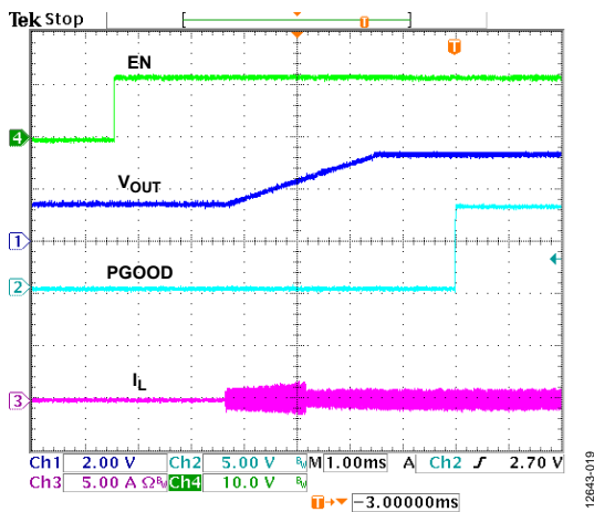
Figure 19. Precharged Output
