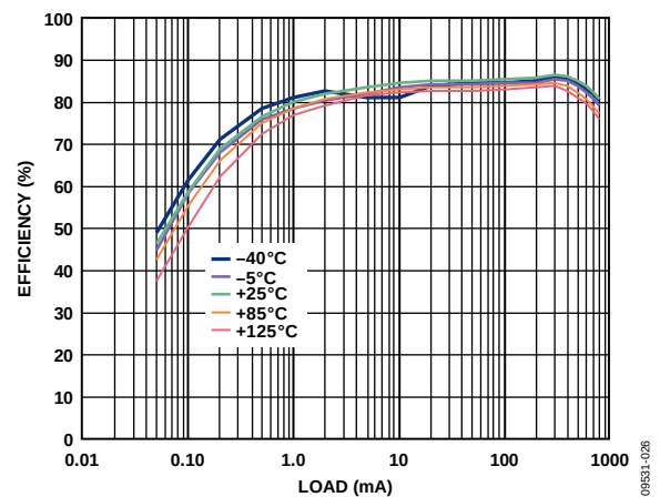
Figure 26. Efficiency vs. Load Current, V_{OUT} = 1.8 V, Different Temperatures, V_{IN} = 4 V
