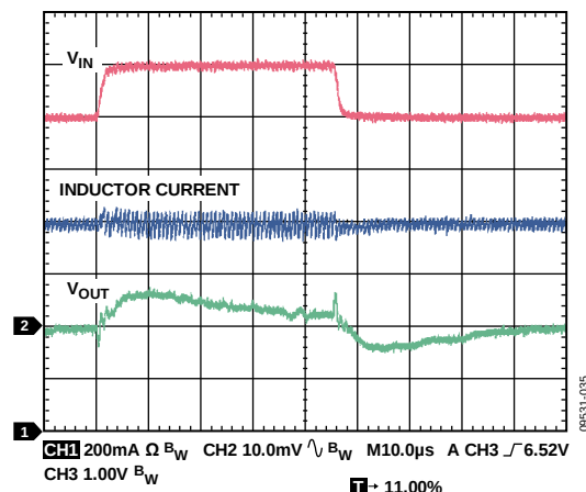
Figure 35. Line Transient, V_{OUT} = 5 V, PWM Mode, 800 mA, V_{IN1} = 6 V to 7 V, 2 µs Rise Time, C_{IN} = 3.3 µF
