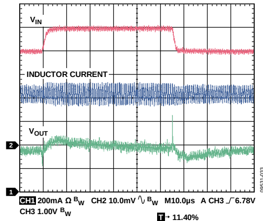
Figure 33. Line Transient, V_{OUT} = 3.3 V, PWM Mode, 800 mA, V_{IN1} = 6 V to 7 V, 2 µs Rise Time, C_{IN} = 3.3 µF
