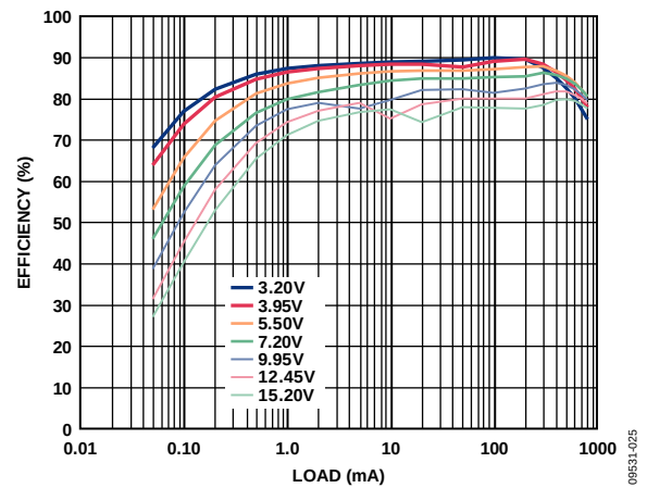
Figure 25. Efficiency vs. Load Current, V_{OUT} = 1.8 V, Different Input Voltages
