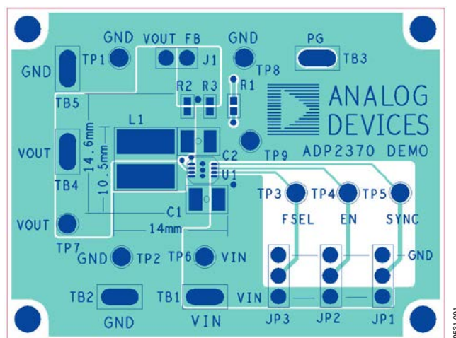
Figure 91. PCB Layout, Top
