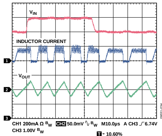
Figure 34. Line Transient, V_{OUT} = 5 V, PSM Mode, 100 mA, V_{IN1} = 6 V to 7 V, 2 µs Rise Time, C_{IN} = 3.3 µF
