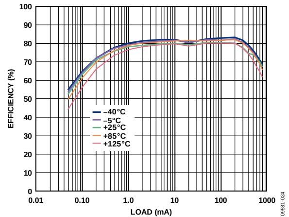
Figure 24. Efficiency vs. Load Current, V_{OUT} = 1.2 V, Different Temperatures, V_{IN} = 4 V
