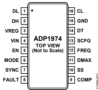
Figure 2. Pin Configuration
