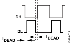
Figure 25. Dead Time ( t_{\text{DEAD}} ) Between DH and DL Transitions
