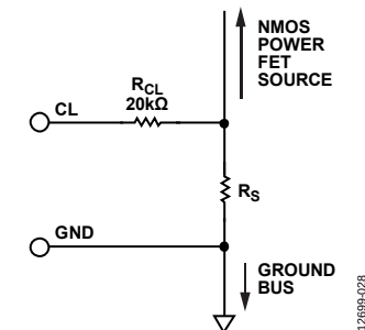
Figure 32. Recommended R_S Kelvin Ground Connection
