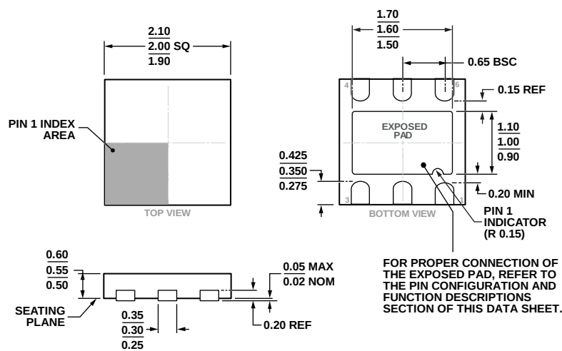
Figure 29. 6-Lead Lead Frame Chip Scale Package [LFCSP_UD] 2.00 mm x 2.00 mm Body, Ultra Thin, Dual Lead (CP-6-3)
