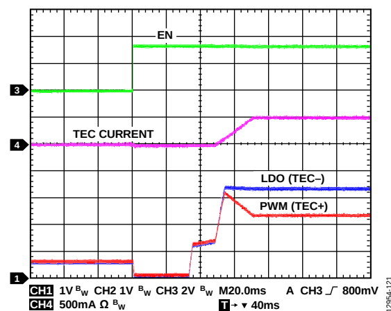
Figure 21. Typical Enable Waveforms in Cooling Mode, V_{IN} = 3.3\text{ V} , Load = 2\ \Omega , TEC Current = 1\text{ A}
