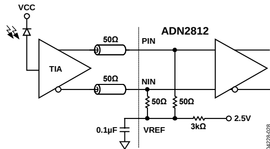
Figure 28. DC-Coupled Application
