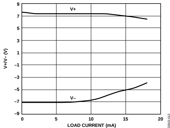
Figure 12. Charge Pump V+ / V- vs. Load Current ( V_{CC} = 3.3 V)
