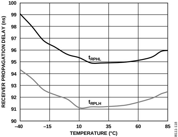
Figure 18. ADM2587E Receiver Propagation Delay vs. Temperature
