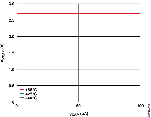
Figure 34. VCAP Voltage ( V_{VCAP} ) vs. VCAP Load ( I_{VCAP} )
