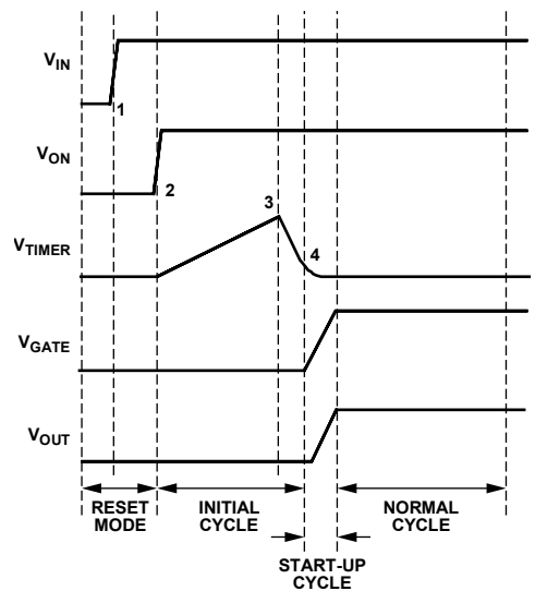
Figure 38. Power-Up Timing
