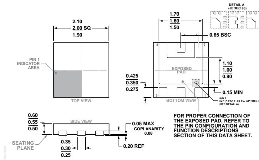
Figure 50. 6-Lead Lead Frame Chip Scale Package [LFCSP] 2.00 mm × 2.00 mm Body and 0.55 mm Package Height (CP-6-7)
