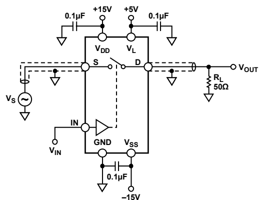
Figure 22. Off Isolation
