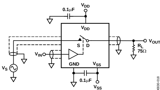
Figure 18. Off Isolation
