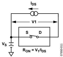
Figure 11. On Resistance
