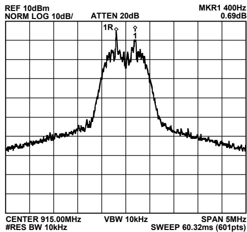
Figure 7. Output Spectrum in FSK Modulation (915 MHz, 172.8 kbps Data Rate, 200 kHz Frequency Deviation)
