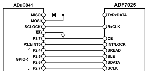
Figure 34. ADuC841 to ADF7025 Connection Diagram
