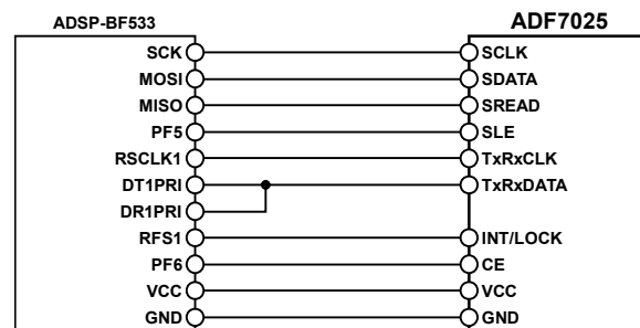
Figure 35. ADSP-BF533 to ADF7025 Connection Diagram
