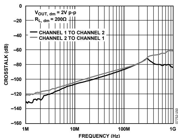
Figure 49. Crosstalk vs. Frequency, ADA4932-2
