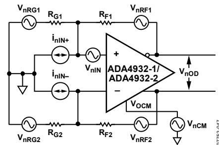
Figure 55. Noise Model
