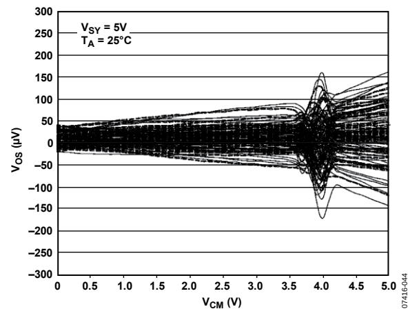
Figure 54. Typical Input Offset Voltage vs. Common-Mode Voltage Response in a Dual Differential Pair Input Stage Op Amp (Powered by a 5 V Supply; Results of Approximately 100 Units per Graph Are Displayed)
