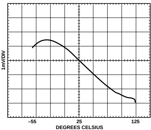
Figure 13. Reference Drift
