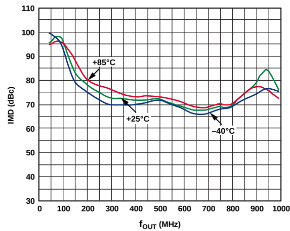
Figure 104. IMD vs. f_{OUT} over Temperature
