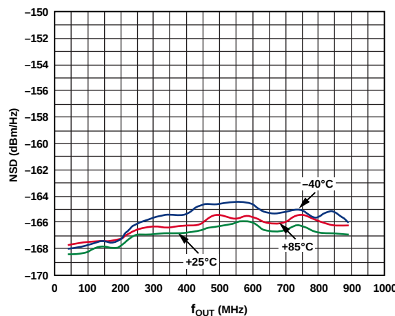
Figure 105. Eight-Tone NSD vs. f_{OUT} over Temperature
