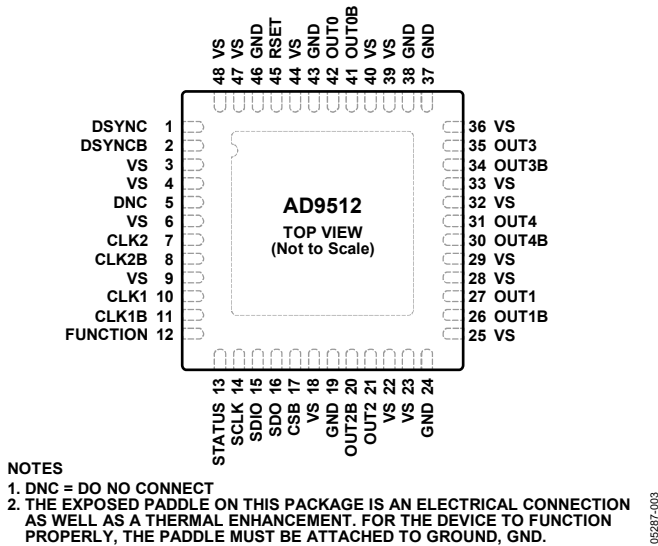
Figure 6. 48-Lead LFCSP Pin Configuration
