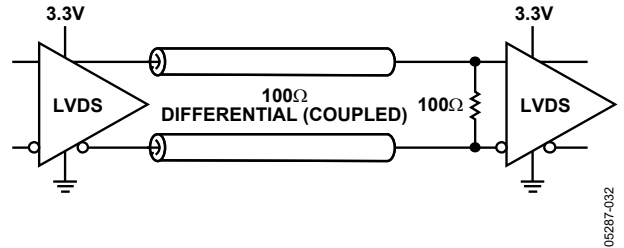
Figure 44. LVDS Output Termination
