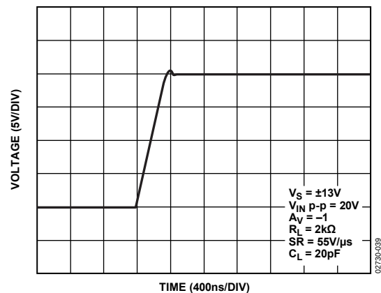
Figure 39. +Slew Rate at G = -1
