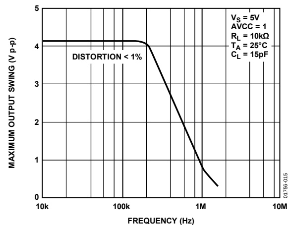
Figure 15. Output Swing vs. Frequency
