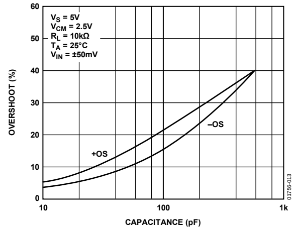
Figure 13. Overshoot vs. Capacitance Load
