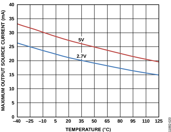
Figure 21. Maximum Output Source Current vs. Temperature
