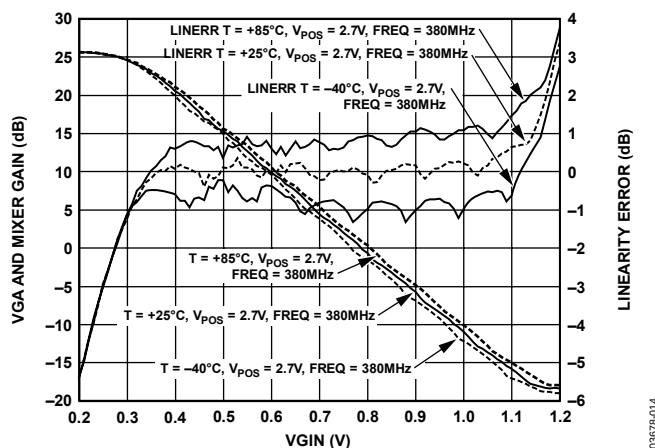
Figure 14. Mixer Gain and Linearity Error vs. VGIN, V_{POS} = 2.7V , F_{IF} = 380\text{ MHz} , F_{BB} = 1\text{ MHz} , Temperature = -40^{\circ}\text{C} , +25^{\circ}\text{C} , +85^{\circ}\text{C}
