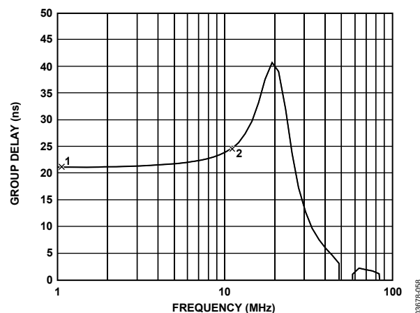
Figure 59. Baseband Filter Group Delay
