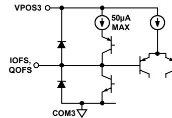
Figure 8. Circuit F
