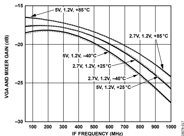
Figure 17. Gain vs. F_{IF} , VGIN = 1.2V , F_{BB} = 1\text{ MHz} , Temperature = -40^{\circ}\text{C} , +25^{\circ}\text{C} , +85^{\circ}\text{C}
