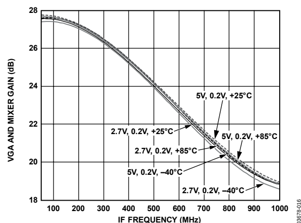
Figure 16. Gain vs. F_{IF} , VGIN = 0.2V , F_{BB} = 1\text{ MHz} , Temperature = -40^{\circ}\text{C} , +25^{\circ}\text{C} , +85^{\circ}\text{C}
