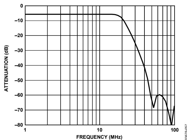
Figure 58. Baseband Filter Response
