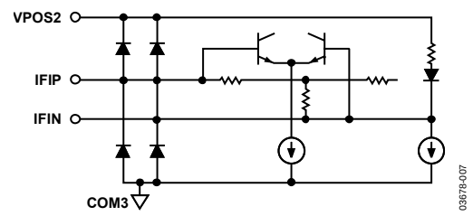
Figure 7. Circuit E
