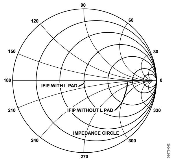
Figure 42. S_{11} of IF Input vs. F_{IF} , F_{IF} = 50\text{ MHz} to 1\text{ GHz} , V_{GIN} = 0.7\text{ V} , V_{POS} = 5\text{ V} (with L Pad, with No Pad, Normalized to 50\Omega )
