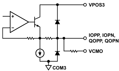
Figure 4. Circuit B
