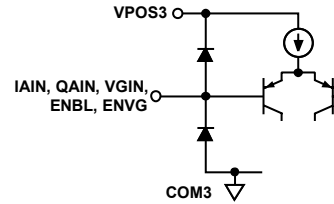
Figure 6. Circuit D
