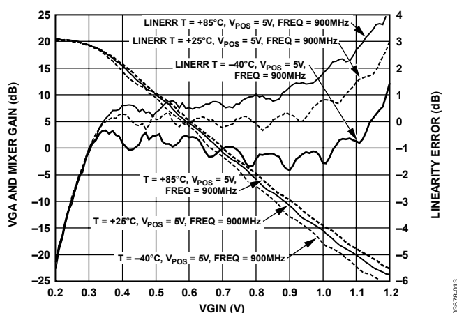
Figure 13. Mixer Gain and Linearity Error vs. VGIN, V_{POS} = 5V , F_{IF} = 900\text{ MHz} , F_{BB} = 1\text{ MHz} , Temperature = -40^{\circ}\text{C} , +25^{\circ}\text{C} , +85^{\circ}\text{C}
