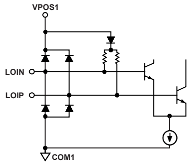
Figure 3. Circuit A
