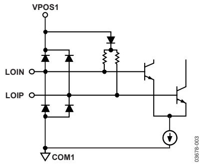
Figure 3. Circuit A
