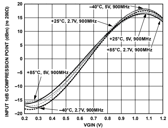
Figure 21. Input 1 dB Compression Point (IP1dB) vs. V_{GIN} , F_{IF} = 900\text{ MHz} , F_{BB} = 1\text{ MHz} , V_{POS} = 2.7\text{ V} , 5\text{ V} , Temperature = -40^{\circ}\text{C} , +25^{\circ}\text{C} , +85^{\circ}\text{C}
