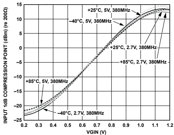
Figure 20. Input 1 dB Compression Point (IP1dB) vs. V_{GIN} , F_{IF} = 380\text{ MHz} , F_{BB} = 1\text{ MHz} , V_{POS} = 2.7\text{ V} , 5\text{ V} , Temperature = -40^{\circ}\text{C} , +25^{\circ}\text{C} , +85^{\circ}\text{C}
