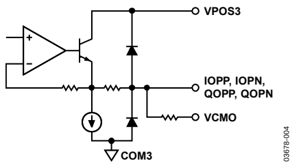
Figure 4. Circuit B
