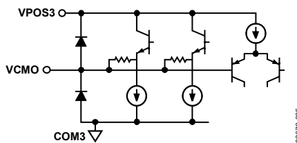
Figure 5. Circuit C
