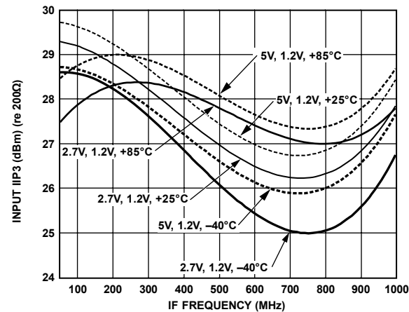
Figure 22. IIP3 vs. F_{IF} , V_{GIN} = 1.2\text{ V} , F_{BB} = 1\text{ MHz} , V_{POS} = 2.7\text{ V} , 5\text{ V} , Temperature = -40^{\circ}\text{C} , +25^{\circ}\text{C} , +85^{\circ}\text{C} , Tone Spacing = 20\text{ kHz}
