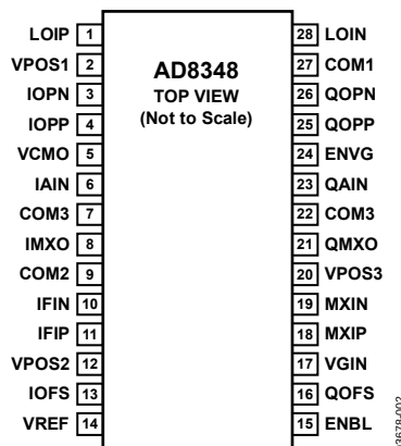
Figure 2. 28-Lead TSSOP Pin Configuration
