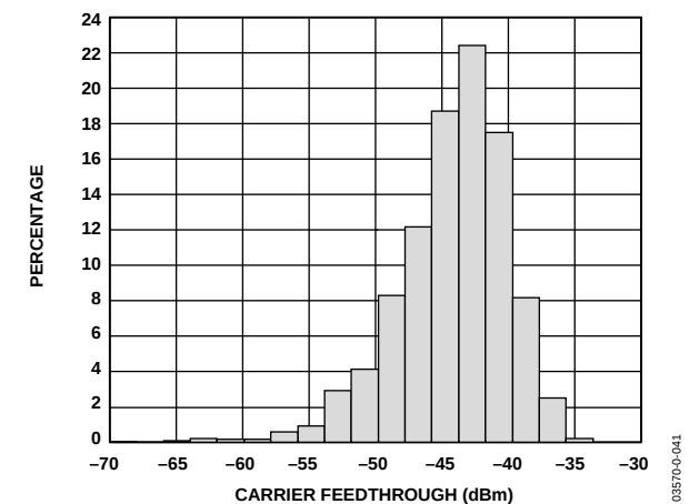
Figure 39. Carrier Feedthrough Distribution at F_{LO} = 2140 MHz ( F_{BB} = 1 MHz, I and Q Inputs Driven in Quadrature at 1.2 V p-p , T_A = 25^\circ\text{C} )
