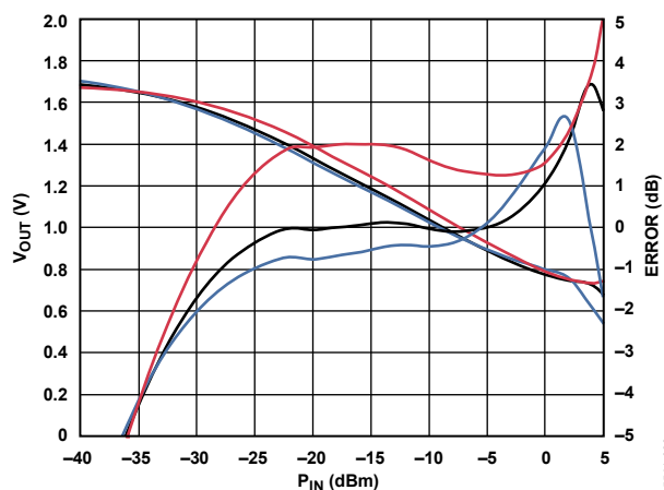
Figure 35. V_{OUT} and Log Conformance vs. Input Amplitude at 10.0 GHz, Multiple Devices, R_{TADJ} = Open, C_{LFP} = 1000 pF
