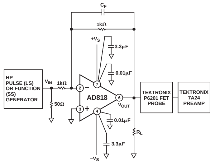
TPC 22. Inverting Amplifier Connection
