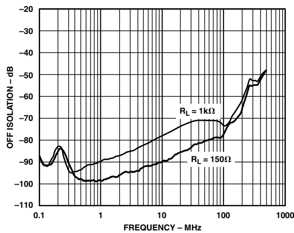
TPC 14. AD8075 Off Isolation vs. Frequency
