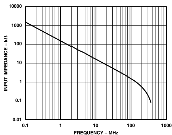
TPC 20. AD8075 Input Impedance vs. Frequency
