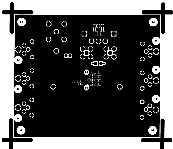
Figure 7. Circuit Side
