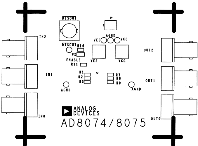
Figure 8. Silkscreen Top
