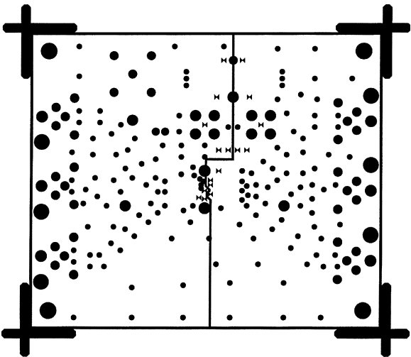
Figure 10. Internal 2
