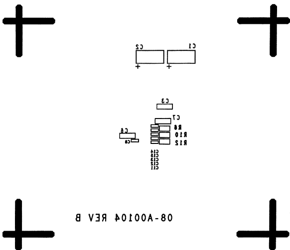
Figure 9. Silkscreen Bottom
