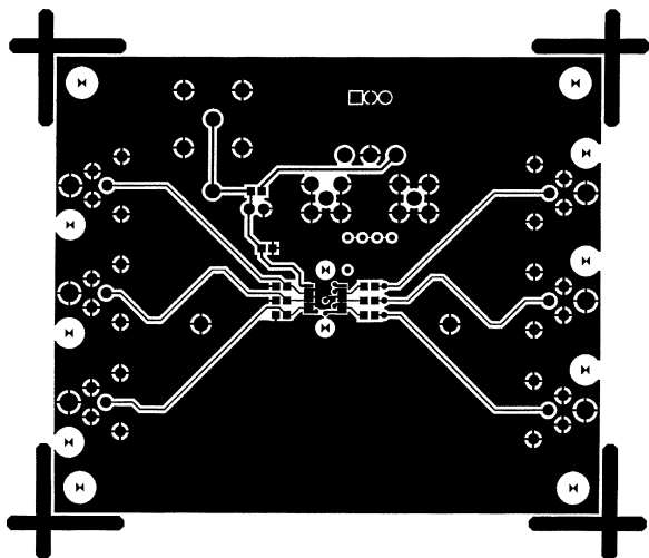
Figure 6. Component Side
