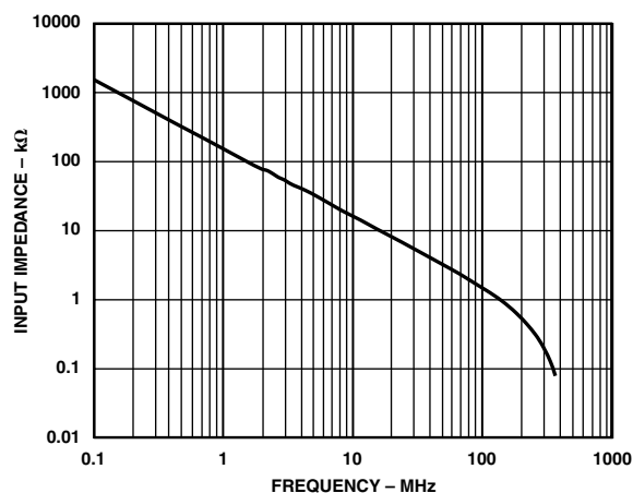
TPC 17. AD8074 Input Impedance vs. Frequency
