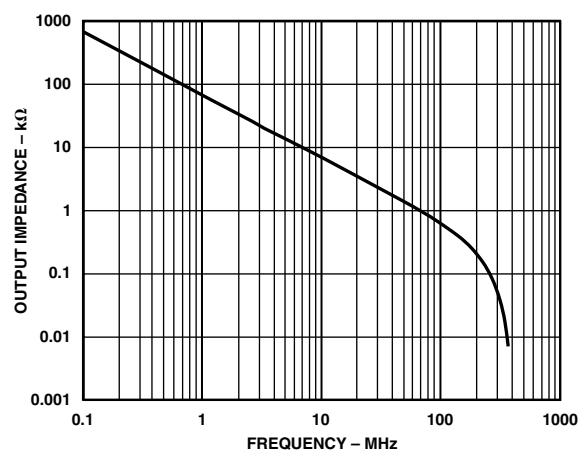
TPC 19. AD8074 Output Impedance vs. Frequency; Disabled
