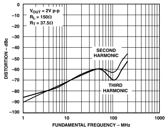
TPC 10. AD8075 Distortion vs. Frequency
