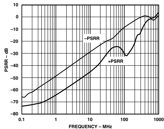
TPC 12. AD8074 PSRR vs. Frequency
