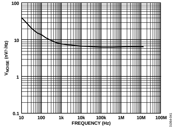
Figure 38. Voltage Noise vs. Frequency
