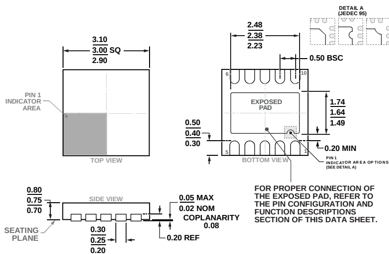
Figure 44. 10-Lead Lead Frame Chip Scale Package [LFCSP] 3 mm × 3 mm Body and 0.75 mm Package Height (CP-10-9) Dimensions shown in millimeters
