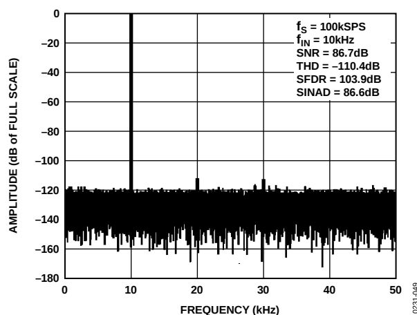
Figure 8. AD7988-1 FFT Plot, VREF = 2.5 V
