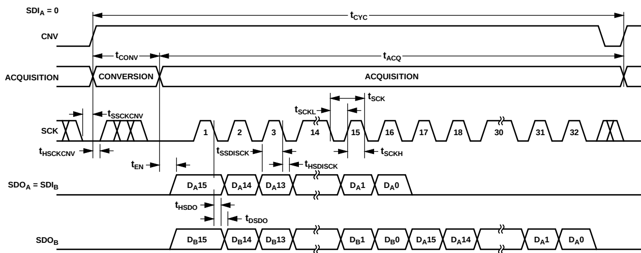
Figure 38. Chain Mode Serial Interface Timing
