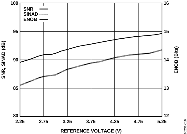
Figure 15. SNR, SINAD, and ENOB vs. Reference Voltage
