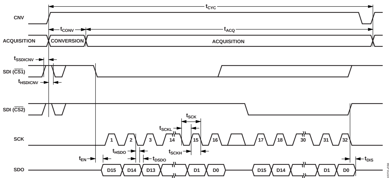
Figure 36. 4-Wire \overline{\text{CS}} Mode Serial Interface Timing
