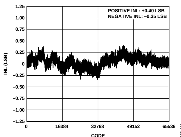
Figure 9. Integral Nonlinearity vs. Code, VREF = 5 V
