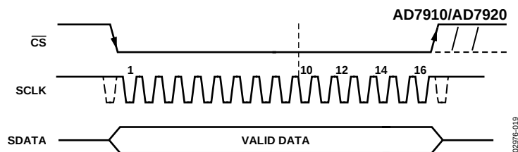
Figure 19. Normal Mode Operation
