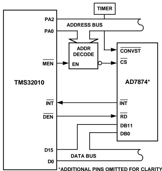
Figure 13. AD7874-TMS32010 Interface
