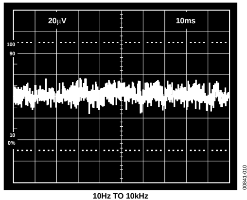
Figure 10. Reduced Noise Performance with C1 = 100 μF, C2 = 100 nF
