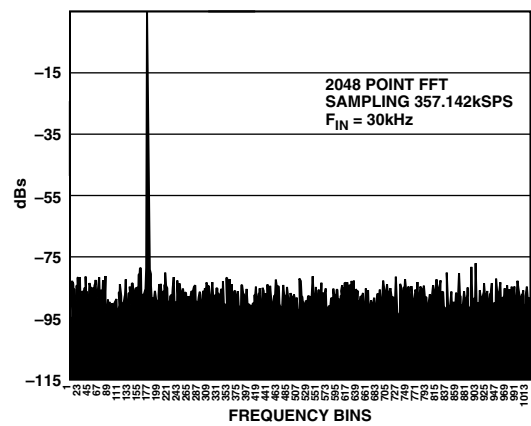
Figure 3. AD7810 SNR
