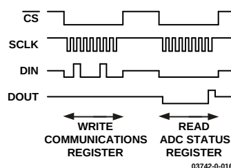
Figure 15. Serial Interface Signals—Registers Access
