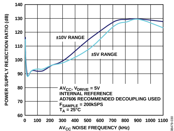
Figure 33. PSRR
