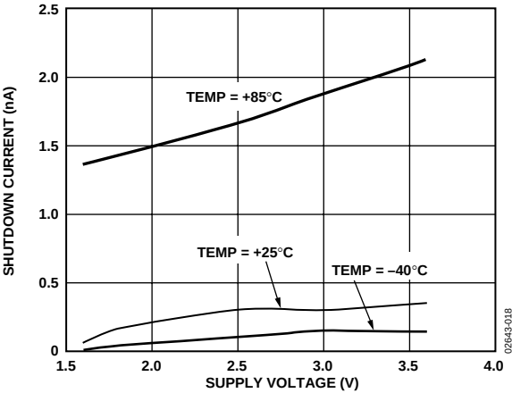
Figure 17. Shutdown Current vs. Supply Voltage
