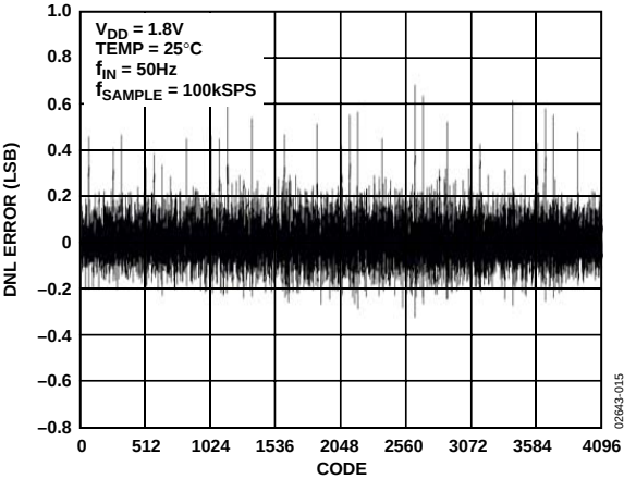
Figure 14. AD7466 DNL Performance
