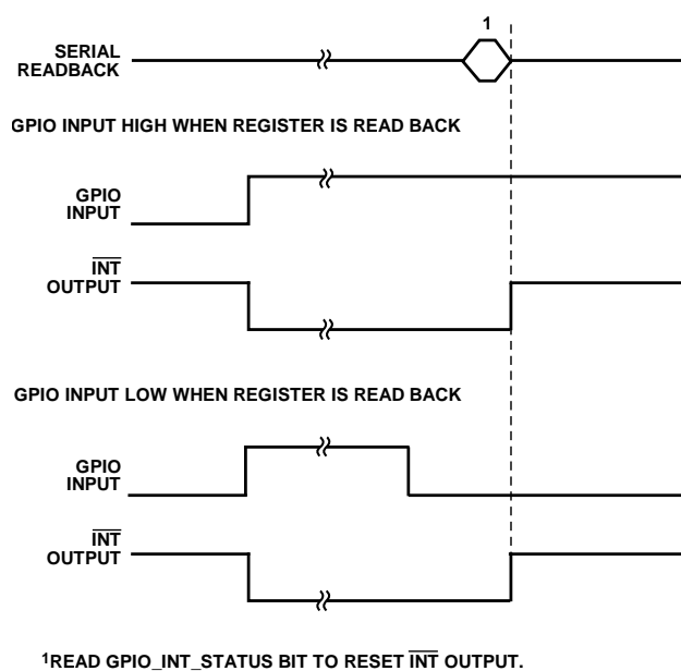
Figure 44. Example of \overline{\text{INT}} Output Controlled by the GPIO Input (GPIO_SETUP = 01, GPIO_INPUT_CONFIG = 01)
