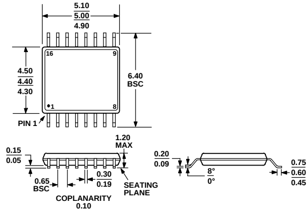
COMPLIANT TO JEDEC STANDARDS MO-153-AB Figure 41. 16-Lead Thin Shrink Small Outline Package [TSSOP] (RU-16) Dimensions shown in millimeters
